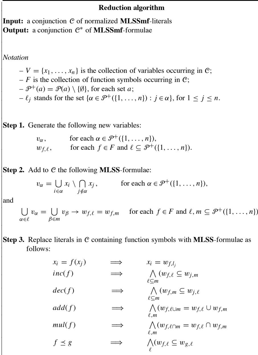
Figure 1: The reduction algorithm.
