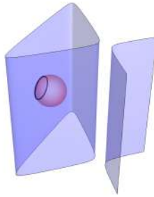
Figure 7: The curve X'_1 .
