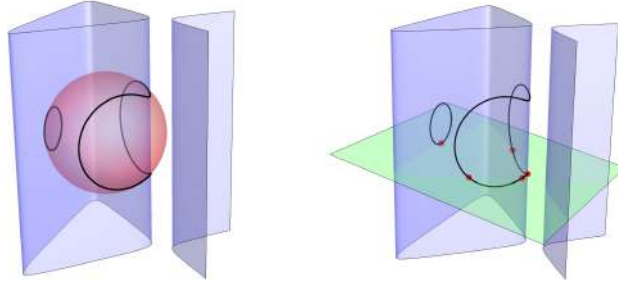
Figure 4: The curve X_2 and its intersection with the plane H_2 .
