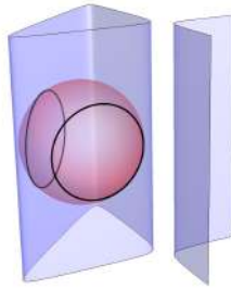
Figure 5: The curve X'_2 .
