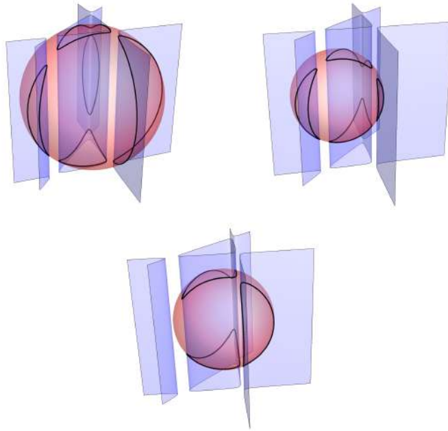
Figure 2: The curves X_5 , X_4 , and X_3 .
