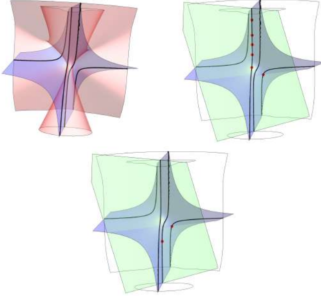
Figure 8: The curve X_{2-4} ; the intersections X_{2-4} \cap H and X_{2-5} \cap H .
