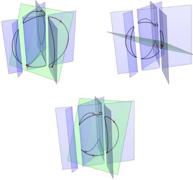
Figure 3: Intersecting curves and planes: X_i \cap H_i for i = 5, 4, 3 .
