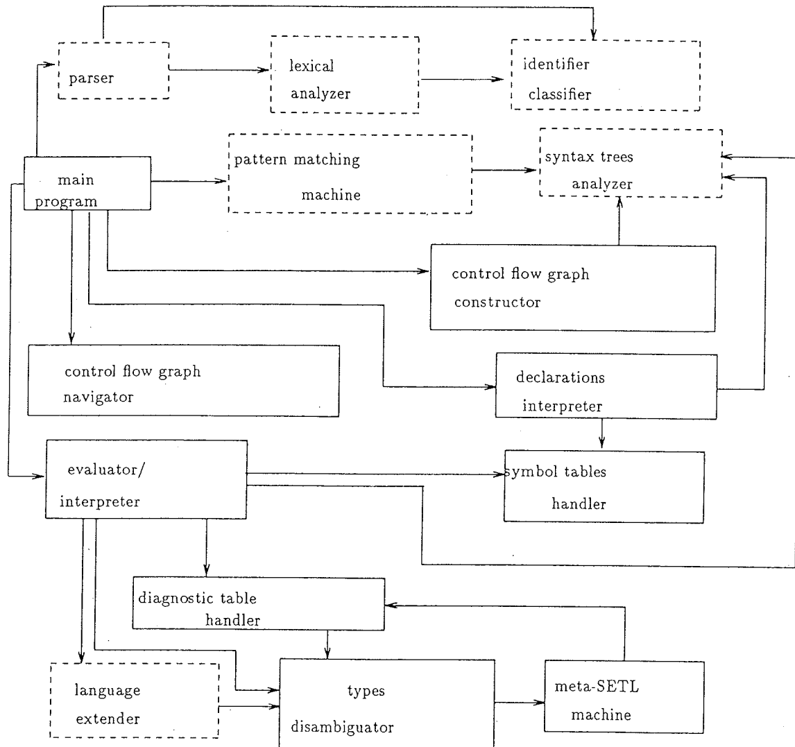
Figure 1 - Meta-interpreter dependency graph.
